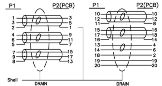
Pin Assignment
